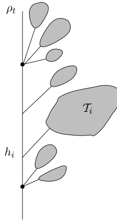
FIG. 2. The measure \rho_t and the family (h_i, \mathcal{T}_i)_{i \in \mathcal{I}} .
