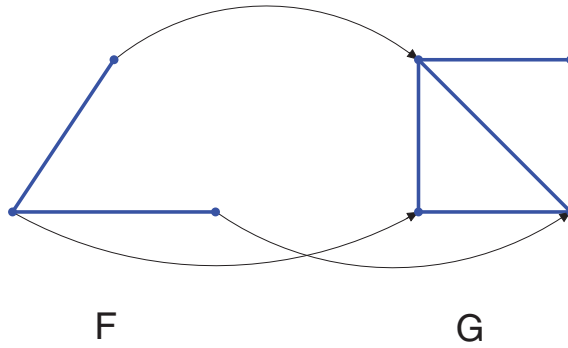
FIGURE 2 An example of an injective homomorphism but not an induced homomorphism [Colour figure can be viewed at wileyonlinelibrary.com]
