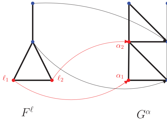
FIGURE 1 Example of an injective homomorphism from partially labeled graphs [Colour figure can be viewed at wileyonlinelibrary.com]
