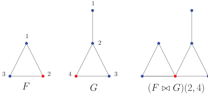
FIGURE 3 Example of two graphs connected by two vertices [Colour figure can be viewed at wileyonlinelibrary.com]
