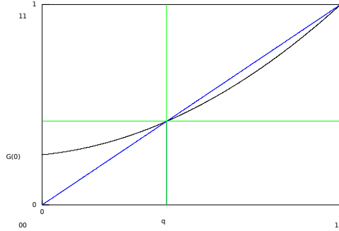
FIGURE 3. The generating functions g_p , g_{\bar{p}} in the lower sub-square and g_{\hat{p}} in the upper sub-square (up to a scaling factor).
