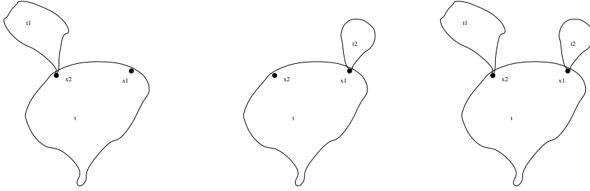
FIGURE 4. Exemple of the third case in (27). The trees are respectively \mathbf{t}_1 , \mathbf{t}_2 , \mathbf{t}_1 \cup \mathbf{t}_2 .
