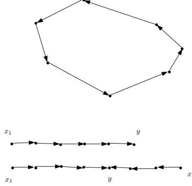
FIGURE 5. The three kinds of weak components of D .
