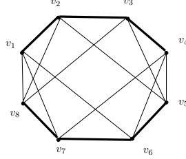
FIGURE 6. The implicit algorithm provided by the proof of Theorem 6 can not improve the bound of this example, 6 edges = (3/4)8 , although the best uncut has 4 edges (v_1v_7, v_2v_8, v_3v_5, v_4v_6) .
