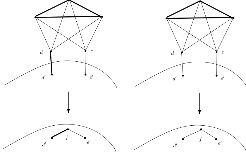
FIGURE 4. The reduction used in the proof of Claim 6.
