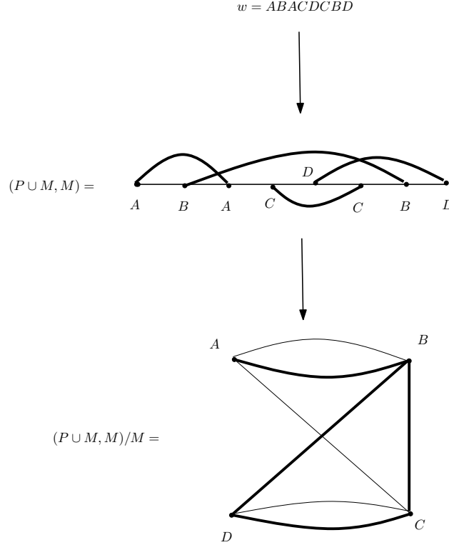
FIGURE 1. Illustration of Proposition 4.
