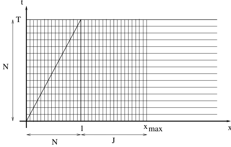
Figure 2: The function g and its domain of computation.
