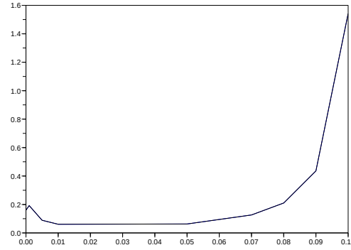
Fig. 5.5. Error as a function of \varepsilon .
