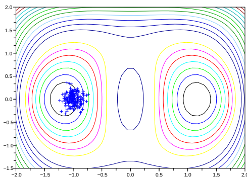
Fig. 5.6. Bad sampling due to a too large value of \varepsilon .
