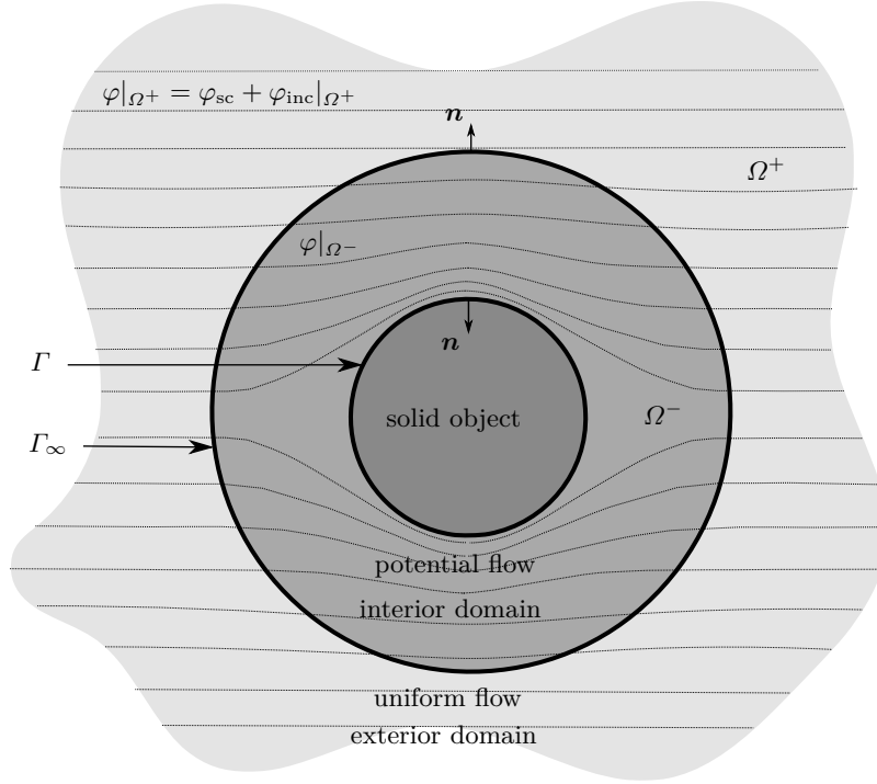
Fig. 3.1. Geometric setup for the coupled problem
