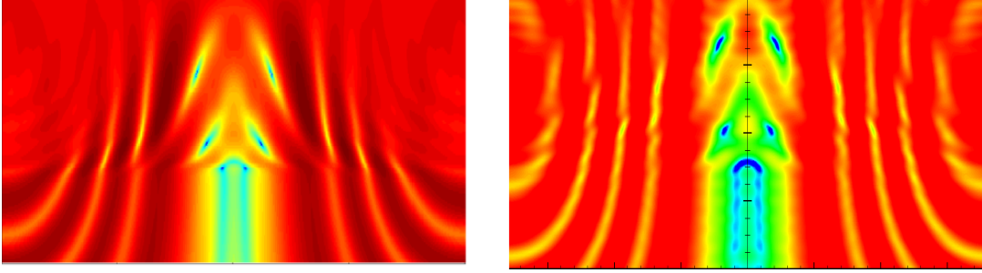
Fig. 4.8. (\text{Pressure}(\text{Jet}) - \text{Pressure}(\text{No Jet}))_{db} with respect to \theta and \phi defined in Figure 4.7, 30 m away from the source. Left: results obtained in [90, 88], right: results obtained using the formulation (3.36)
