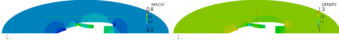
Fig. 4.15. Simplified engine: computed potential flow such that M_M = 0.42 and M_\infty = 0.3 (left: Mach number, right: density).
