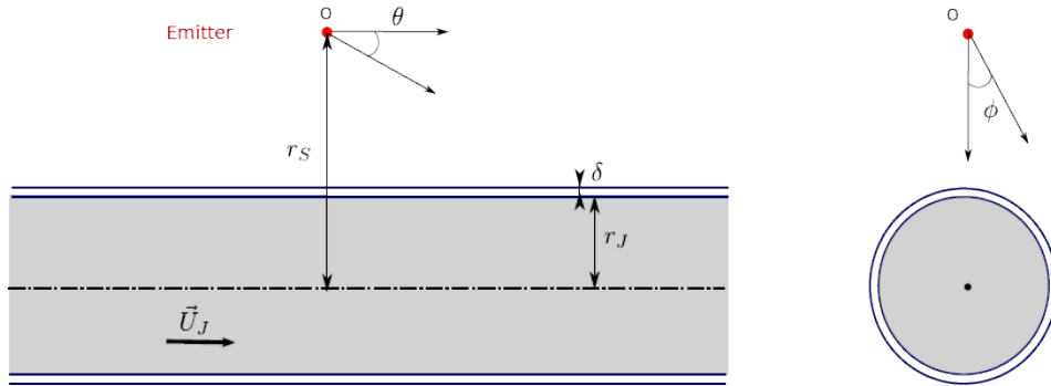
Fig. 4.7. Geometry of the test case
