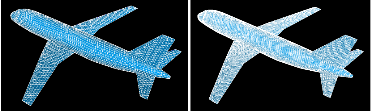
Fig. 6.3. Airbus A319: Mesh 1 and Mesh 2.
