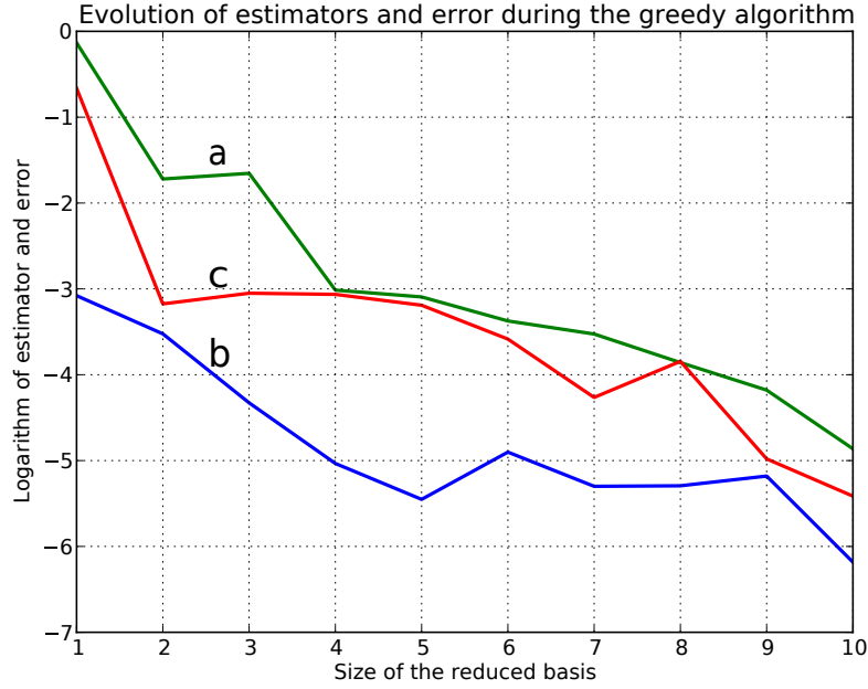
Fig. 8.12. Evolution of the maximum error estimate \Delta_\mu for \mu \in \mathcal{D}_{\text{trial}} (a), the corresponding value of the error |s_\mu^{\text{RB},*\text{RB}} - s_\mu^{\text{FE}}| (b) and the error estimate \Delta_{\hat{\mu}} for \hat{\mu} \in \mathcal{D} taken randomly (c)
