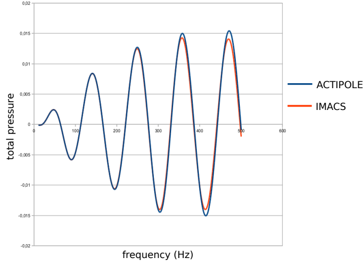
Fig. 4.5. Real part of the difference between the pressure computed at the visualization point and the reference with respect to the frequency of the source - blue: formulation (3.36), red: IMACS.
