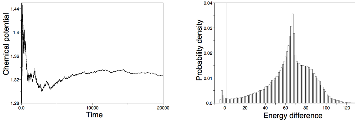
Figure A.3 – Left: Estimate of the chemical potential as a function of time, using the estimator (A.11). Right: Distribution of the free energy differences. Image from [Lelièvre et al., 2010].
