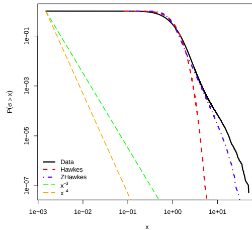
FIGURE 4.5 – Cumulative density function of the Rogers-Satchell volatility for US stock data (plain line), simulated Hawkes data (red dashed line), and simulated ZHawkes data (blue dot-dashed line).
