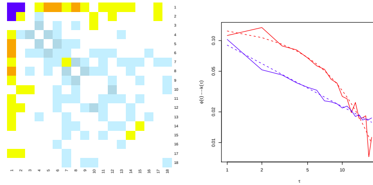
FIGURE 4.3 – Fit of the kernel K by the sum of a power-law diagonal matrix and an exponential rank-one matrix. Left : heatmap of the difference between the fitted matrix and the original one. The coefficients are small (white or lightly-colored) except for the upper-left corner : the original matrix features a stronger short-term feedback. Right : kernels \phi(\tau) and k(\tau) that minimize the matrix distance \sum [K(\tau, \tau') - \phi(\tau)\delta_{\tau-\tau'} - k(\tau)k(\tau')]^2 . The rank-one kernel k is plotted in red (and is larger for small \tau 's), and the diagonal kernel \phi is plotted in blue, both in log-log scale. The dashed lines are the power-law fit for \phi(\tau) with exponent 0.6, and the exponential fit for k(\tau) with characteristic time about 30 min.
