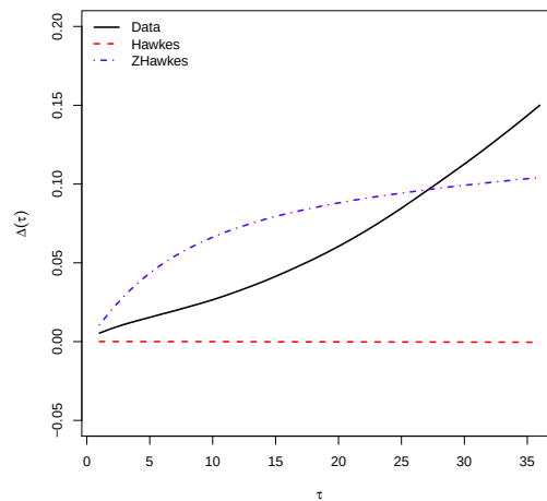
FIGURE 4.7 – Time asymmetry ratio \Delta(\tau) for US stock data (plain line), simulated Hawkes data (red dashed line), and simulated ZHawkes data (blue dot-dashed line).
