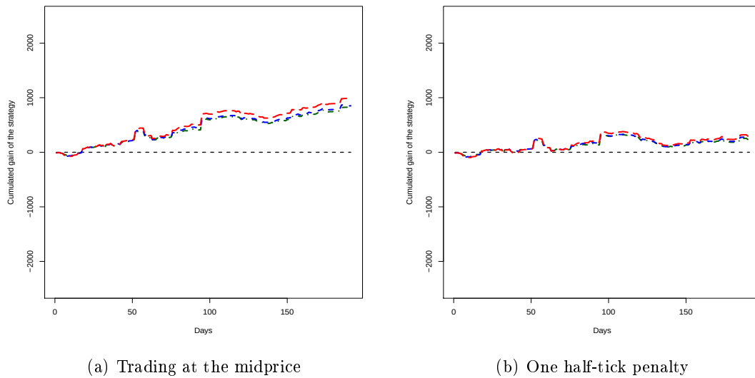
FIGURE 2.6 – Cumulated gains of the strategy applied on BNP Paribas on the period January-September 2013, every day between 11.30a.m. and 1p.m. The (red) long-dashed line is the performance of the Poisson model, the (blue) dashed line is the mono-exponential Hawkes model, and the (green) dot-dashed line is the multi-exponential Hawkes model. Left : we allow the strategy to trade at the midprice. Right : we apply a posteriori a linear cost penalty of one half-tick to account for the bid-ask spread.
