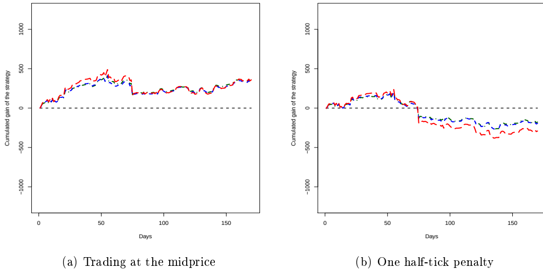
FIGURE 2.4 – Cumulated gains of the strategy applied on BNP Paribas on the period February-September 2012, every day between 11.30a.m. and 1p.m. The (red) long-dashed line is the performance of the Poisson model, the (blue) dashed line is the mono-exponential Hawkes model, and the (green) dot-dashed line is the multi-exponential Hawkes model. Left : we allow the strategy to trade at the midprice. Right : we apply a posteriori a linear cost penalty of one half-tick to account for the bid-ask spread.
