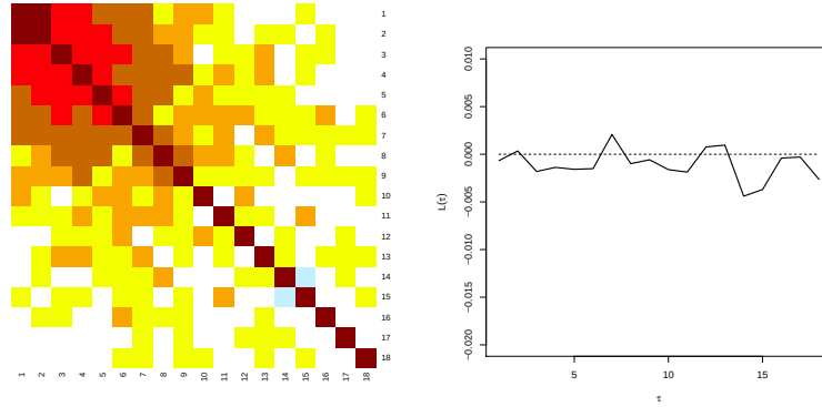
FIGURE 4.1 – QARCH kernels calibrated on five-minute intra-day returns for US stocks. The maximum lag is 18 bins, i.e. one hour and a half of trading time. Left : heatmap of the quadratic kernel. White coefficients are close to zero, blue ones are negative and yellow/orange/red ones are positive, with darker shades as they increase in absolute value. We see that all the significant coefficients are positive, with a non-negligible off-diagonal component. Right : leverage kernel. It is hardly distinct from zero and can be considered as pure noise (as opposed to daily models where it is significantly negative).
