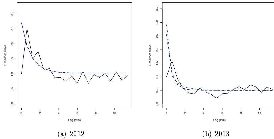
FIGURE 2.1 – The estimated propagator for BNP Paribas. The plain line is the unconstrained propagator, the (blue) dashed line is the mono-exponential resilience curve, and the (green) dot-dashed line is the multi-exponential resilience curve.
