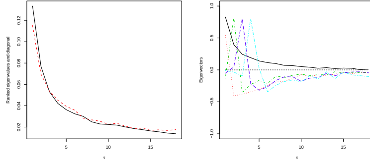
FIGURE 4.2 – Spectral decomposition of the quadratic QARCH kernel. Left : ranked eigenvalues (plain dark line) and diagonal coefficients (dashed). One can see that the diagonal coefficients are very close to the eigenvalues, except for the first eigenvalue which is significantly larger than the maximum of the diagonal. Right : eigenvectors corresponding to the five largest eigenvalues. The first eigenvector (plain dark line) is a positive decaying kernel, the others are close to the canonical vectors e_i(\tau) = \delta_{i-\tau} .
