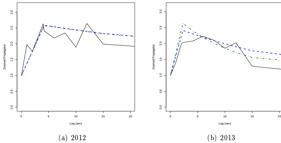
FIGURE 2.2 – Zoom on the first twenty seconds of the propagator curve for BNP Paribas. The plain line is the unconstrained curve, the (blue) dashed line is the mono-exponential curve, and the (green) dot-dashed line is the multi-exponential curve. The propagator is increasing during a few seconds, before the resilience effect kicks in.
