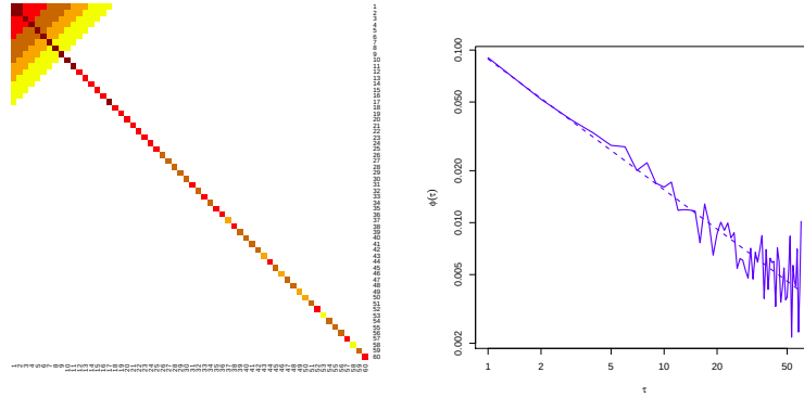
FIGURE 4.4 – Long-range kernel K . Left : heatmap of the long-range kernel, with the off-diagonal fixed as its exponential rank-one fit, and with the diagonal calibrated with no constraints. Right : long-range kernel \phi_{lr}(\tau) = K(\tau, \tau) - k^2(\tau) . The kernel \phi(\tau) is plotted in log-log scale, with its power-law fit with exponent 0.76 (dashed).
