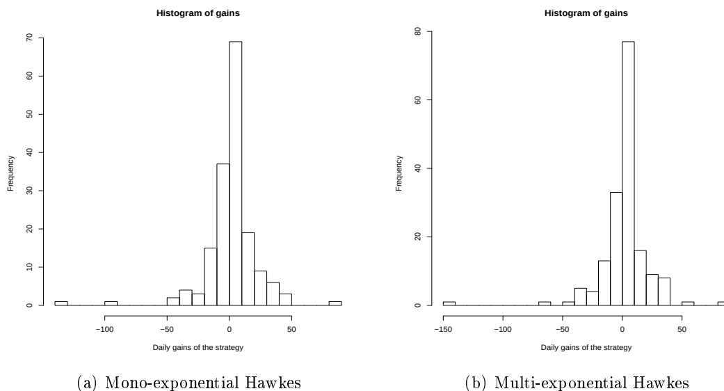
FIGURE 2.5 – Histogram of the daily gains of the strategy applied on BNP Paribas on the period February-September 2012, between 11.30a.m. and 1p.m. Left : Mono-exponential Hawkes model. Right : Multi-exponential Hawkes model.
