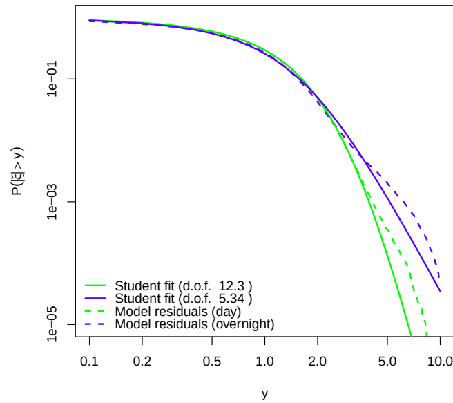
FIGURE 3.6 – CDF \mathbb{P}(|\xi| > y) of the residuals \xi^D and \xi^N , in log-log scale.
