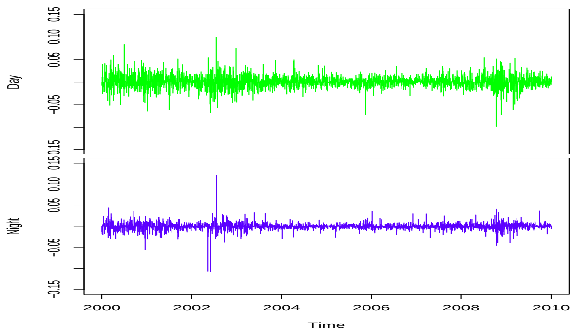
FIGURE 3.1 – Example of a historical time series of stock day returns (top) and overnight returns (bottom).
