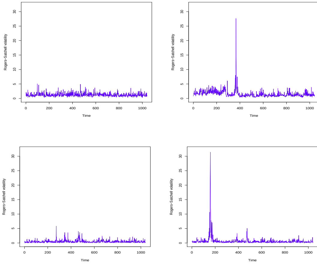
FIGURE 4.6 – Time series of Rogers-Satchell volatility. Above : real data ; below : simulated ZHawkes data ; left : period of calm ; right : cluster of intense activity.
