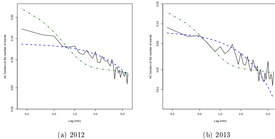
FIGURE 2.3 – Auto-correlation function of the number of midpoint moves triggered by trades (plain line), in log-log scale, for BNP Paribas. The (blue) dashed line is the auto-correlation generated by the mono-exponential Hawkes model, the (green) dot-dashed line is generated by the multi-exponential Hawkes model.
