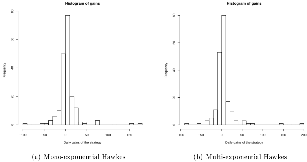
FIGURE 2.7 – Histogram of the daily gains of the strategy applied on BNP Paribas on the period January-September 2013, between 11.30a.m. and 1p.m. Left : Mono-exponential Hawkes model. Right : Multi-exponential Hawkes model.
