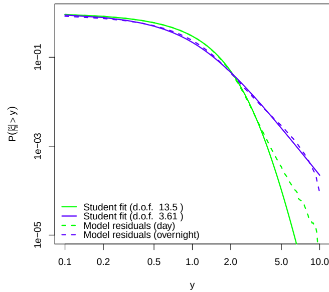
FIGURE 3.4 – CDF \mathbb{P}(|\xi| > y) of the residuals \xi^D and \xi^N , in log-log scale.
