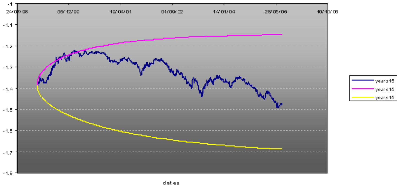
back-testing taux 15ans
