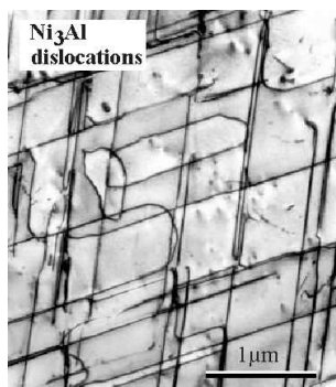
FIGURE 1. Dislocation lines in Nickel Aluminium alloy.
