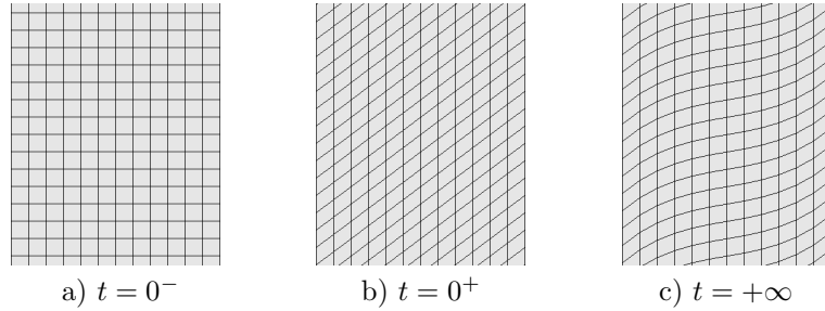
FIGURE 5. Deformation of a slab for model (23)
