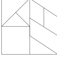
FIGURE 1. An example of admissible mesh
