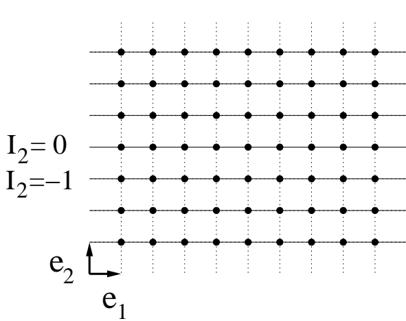
Figure 1: Perfect crystal
