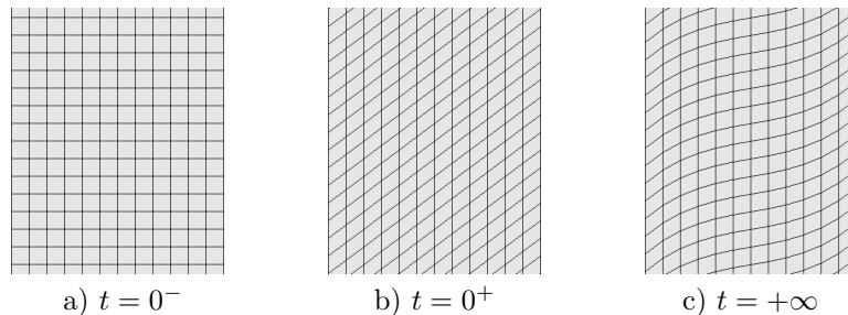
Figure 5: Deformation of a slab for model (4.9)
