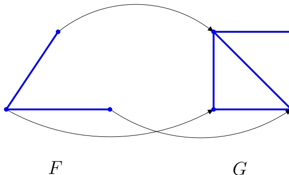
FIGURE 2. An example of an injective homomorphism but not an induced homomorphism.
