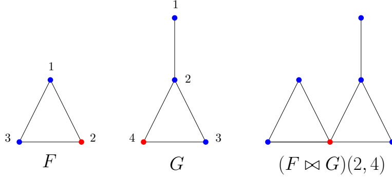
FIGURE 3. Example of two graphs connected by two vertices.
